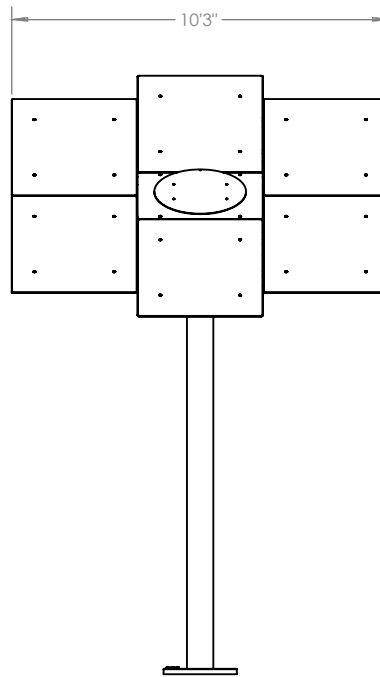
Array shown at 25 degree angle, no Twist. Dimensions will vary with site-specific Tilt and Twist orientation.
