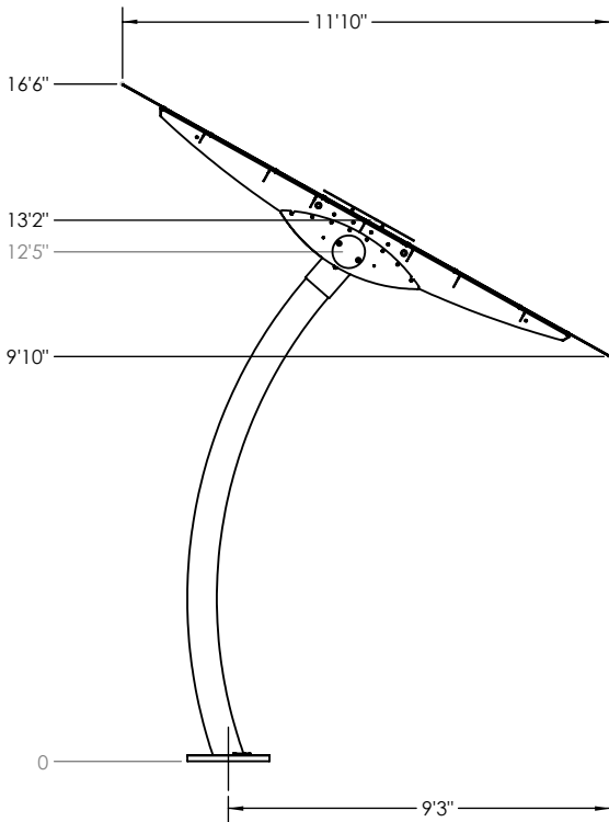
Array shown at 25 degree angle, no Twist. Dimensions will vary with site-specific Tilt and Twist orientation.
